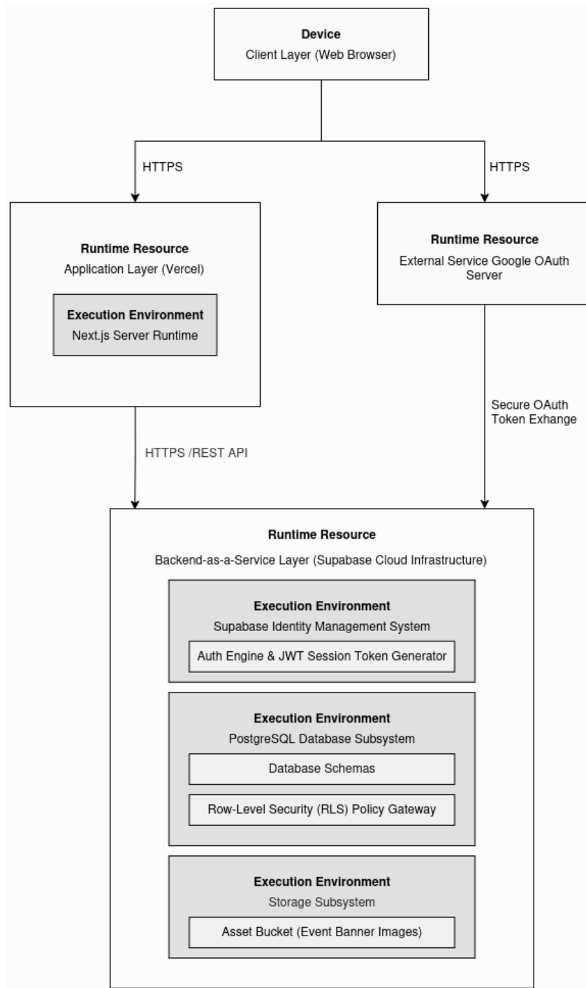
Figure 37: Deployment View
